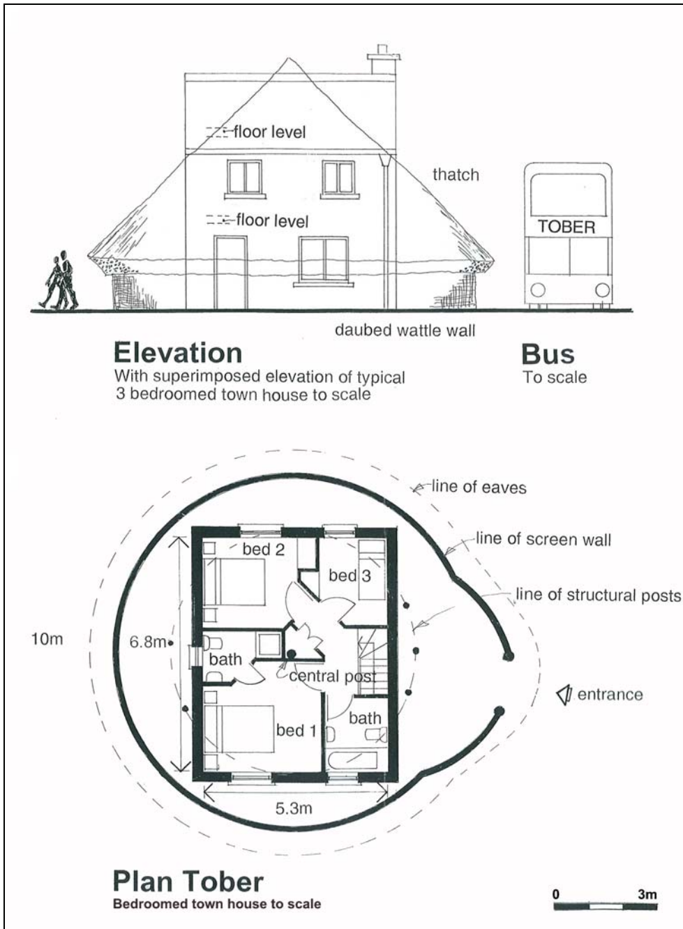
Illus. Reconstruction of Tober house with super-imposed elevation and floor-plan of modern townhouse and double-decker bus for scale (Allman 2009)
